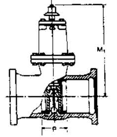
Push-On Ends For PVC Pipe C566/F-5072
